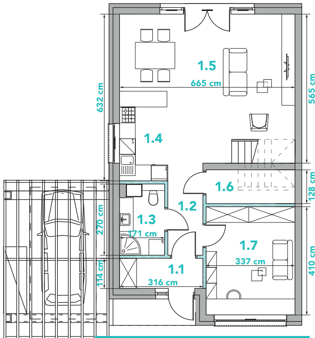
Parter 67,59 m 2
